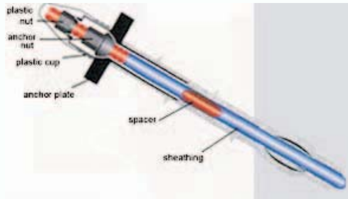
Temporary anchor
