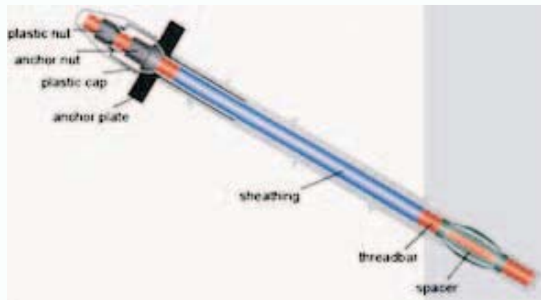
DCP anchor (Double Corrosion Protection)
